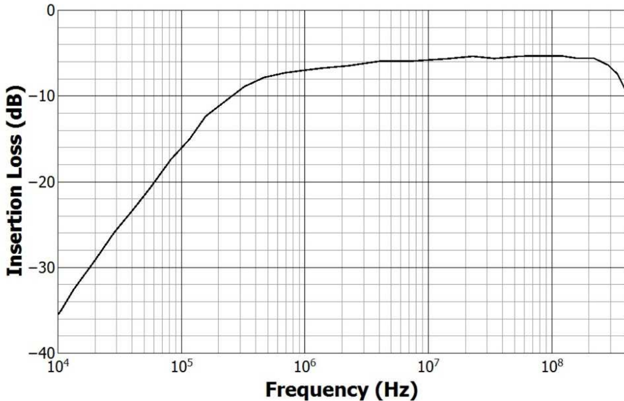
Model 8700i
